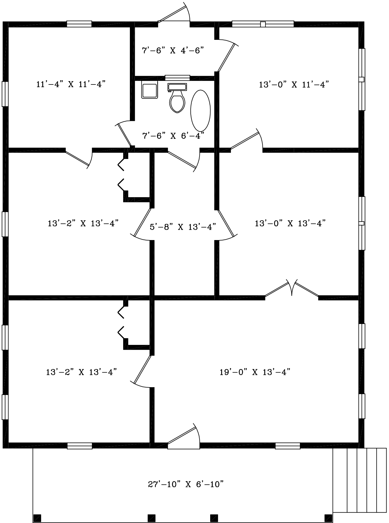
BEIGE HOUSE 178 Main Street 1342 S.F.
